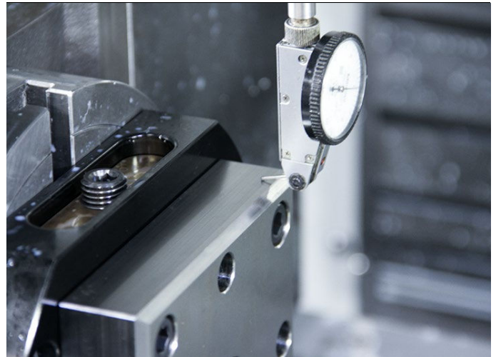
Precision milled sides allow for indication of center line.
