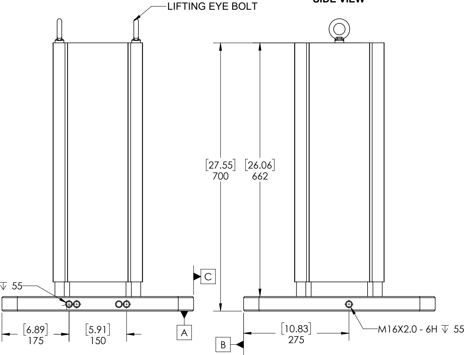
FRONT VIEW
