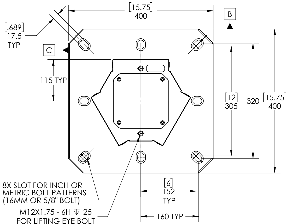
BOTTOM VIEW
