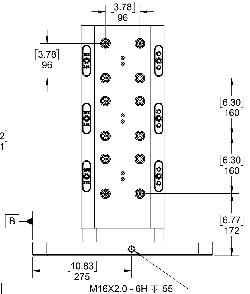
SIDE VIEW
