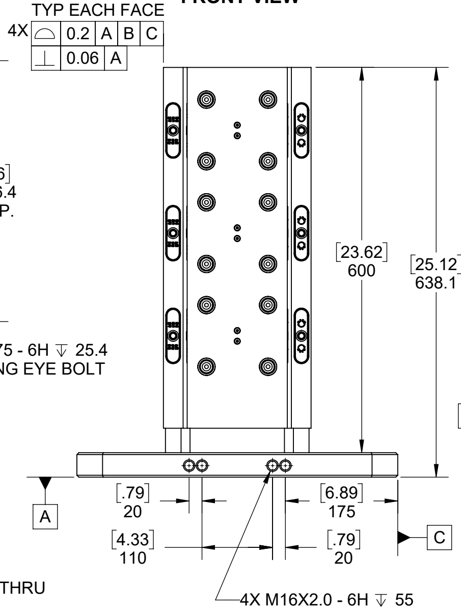
FRONT VIEW
