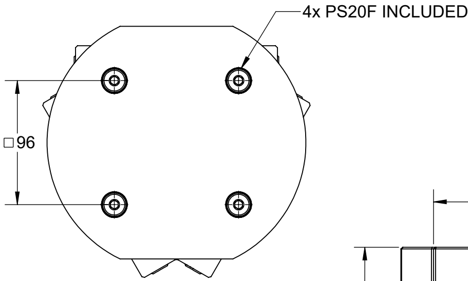
BOTTOM VIEW
