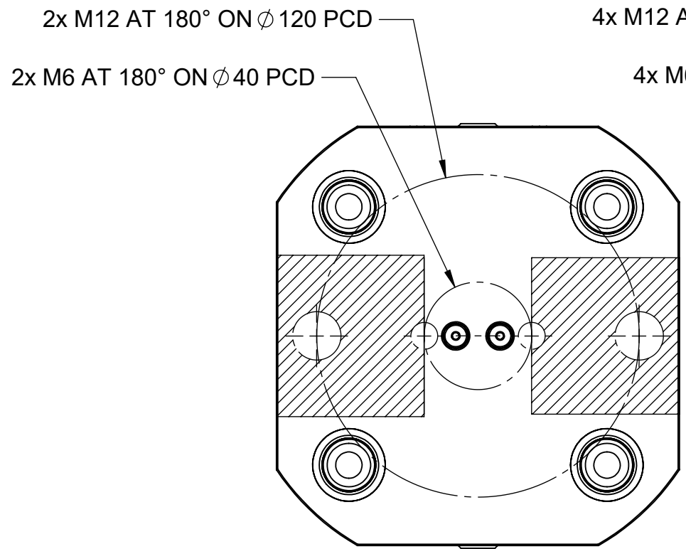
180° PATTERN
