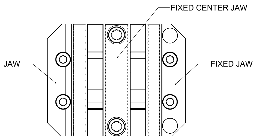
JAW MOUNTING
