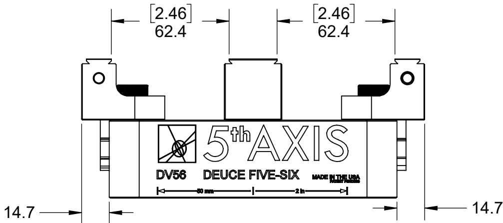
REVERSE JAWS (MAXIMUM CLAMPING RANGE)
