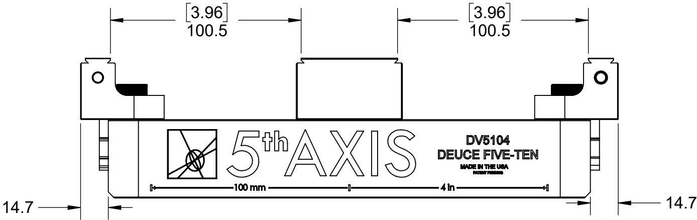
REVERSE JAWS (MAXIMUM CLAMPING RANGE)
